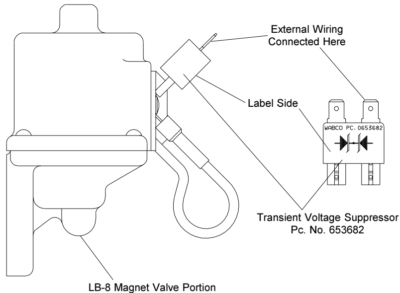
Figure 1 - LB-8 Magnet Valve Portion with Transient Voltage Suppressor
